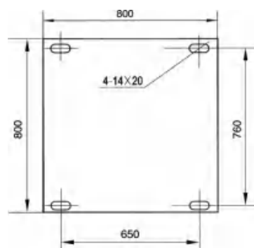
Installation dimension of Ring Main cabinet
