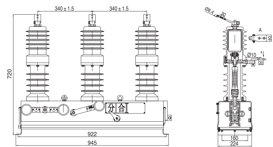
Diagram 1 ZW32-12 Outdoor high voltage vacuum circuit breaker
