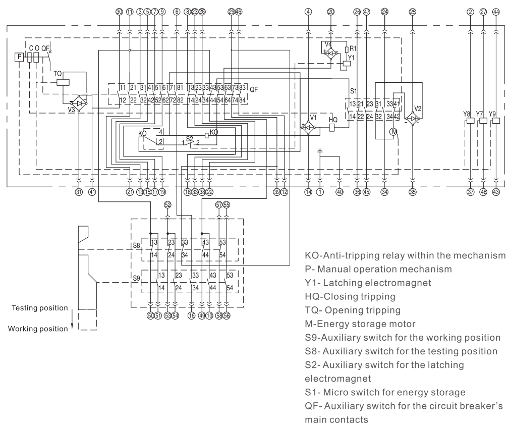
Diagram 2 Inner electrical principal diagram for the withdrawable circuit breaker (with anti-trip, latching, over-current)
